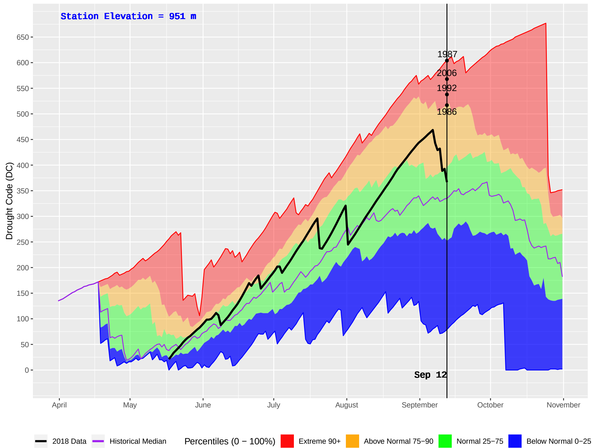
NORTH BABINE (173) : Historical (1986–2016) and Current (2018) Daily Drought Code (DC)
