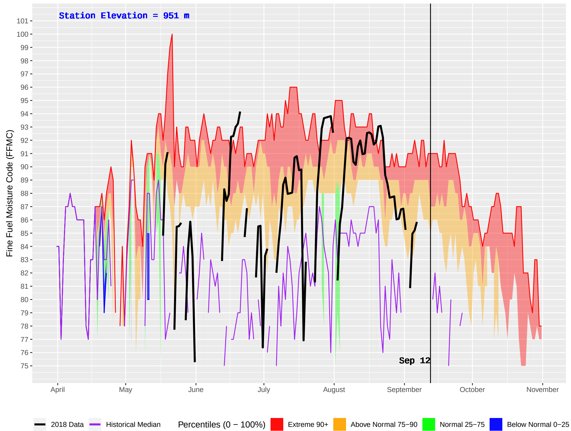
NORTH BABINE (173) : Historical (1986–2016) and Current (2018) Daily Fine Fuel Moisture Code (FFMC)
