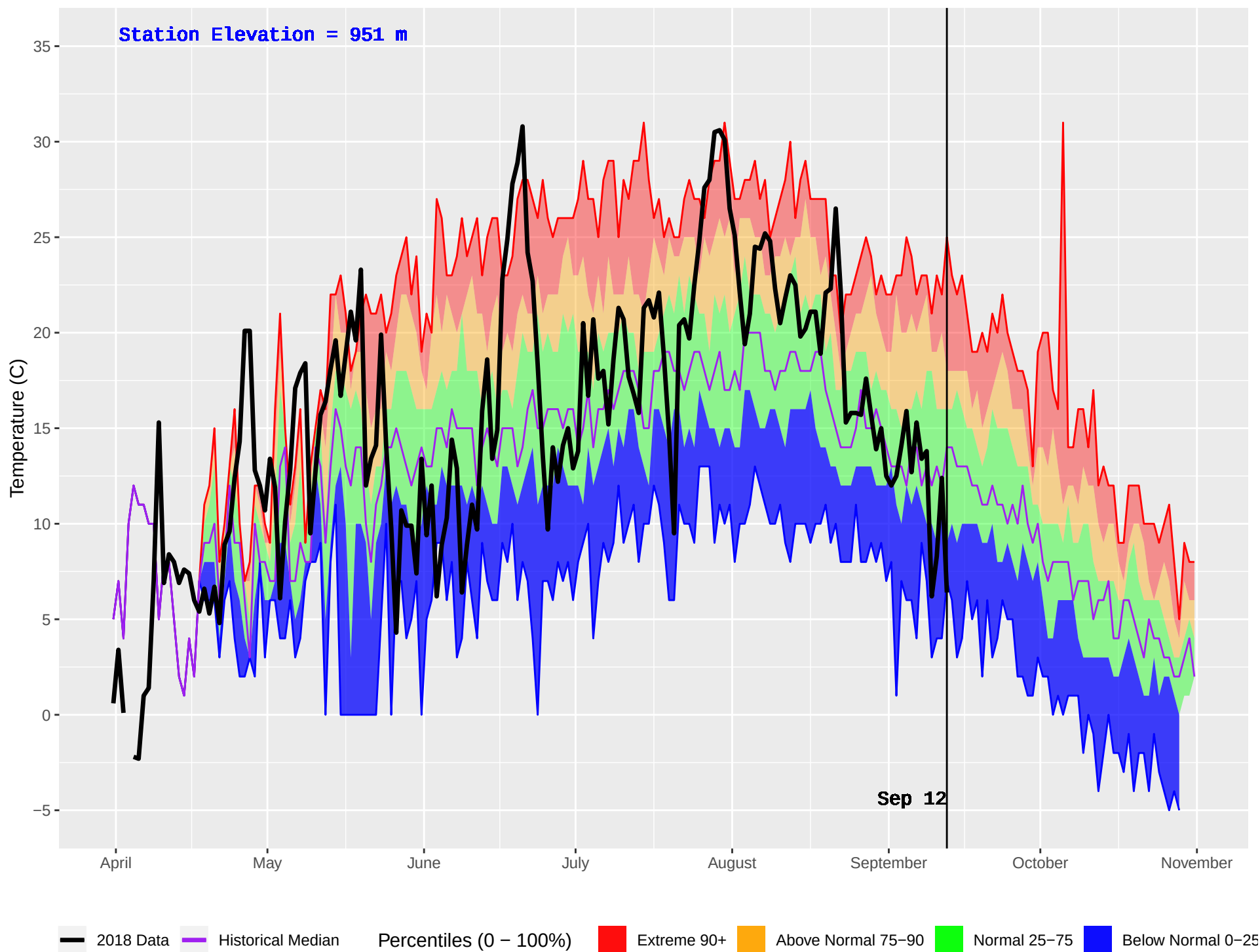
NORTH BABINE (173) : Historical (1986–2016) and Current (2018) Daily Temperature
