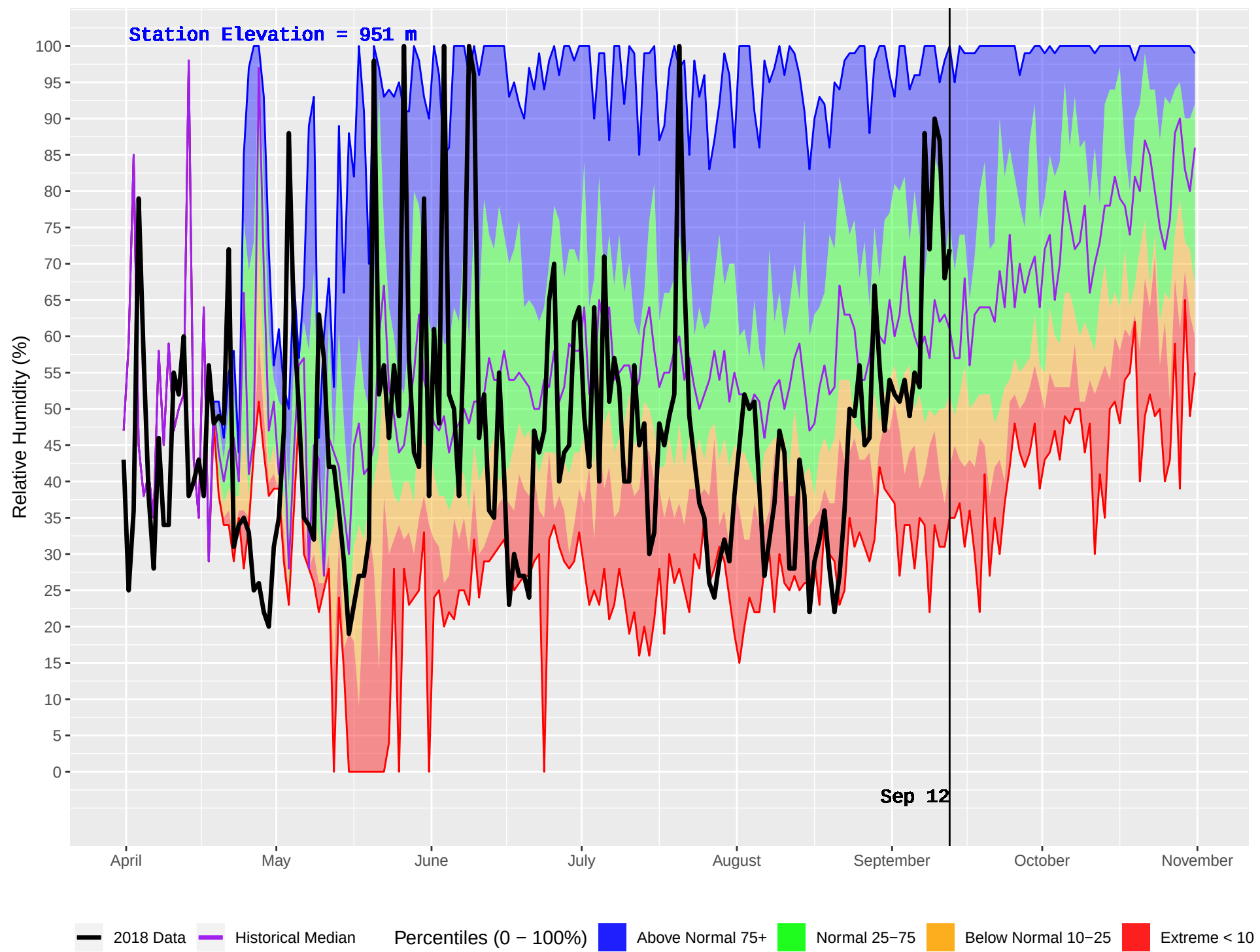
NORTH BABINE (173) : Historical (1986–2016) and Current (2018) Daily Relative Humidity
