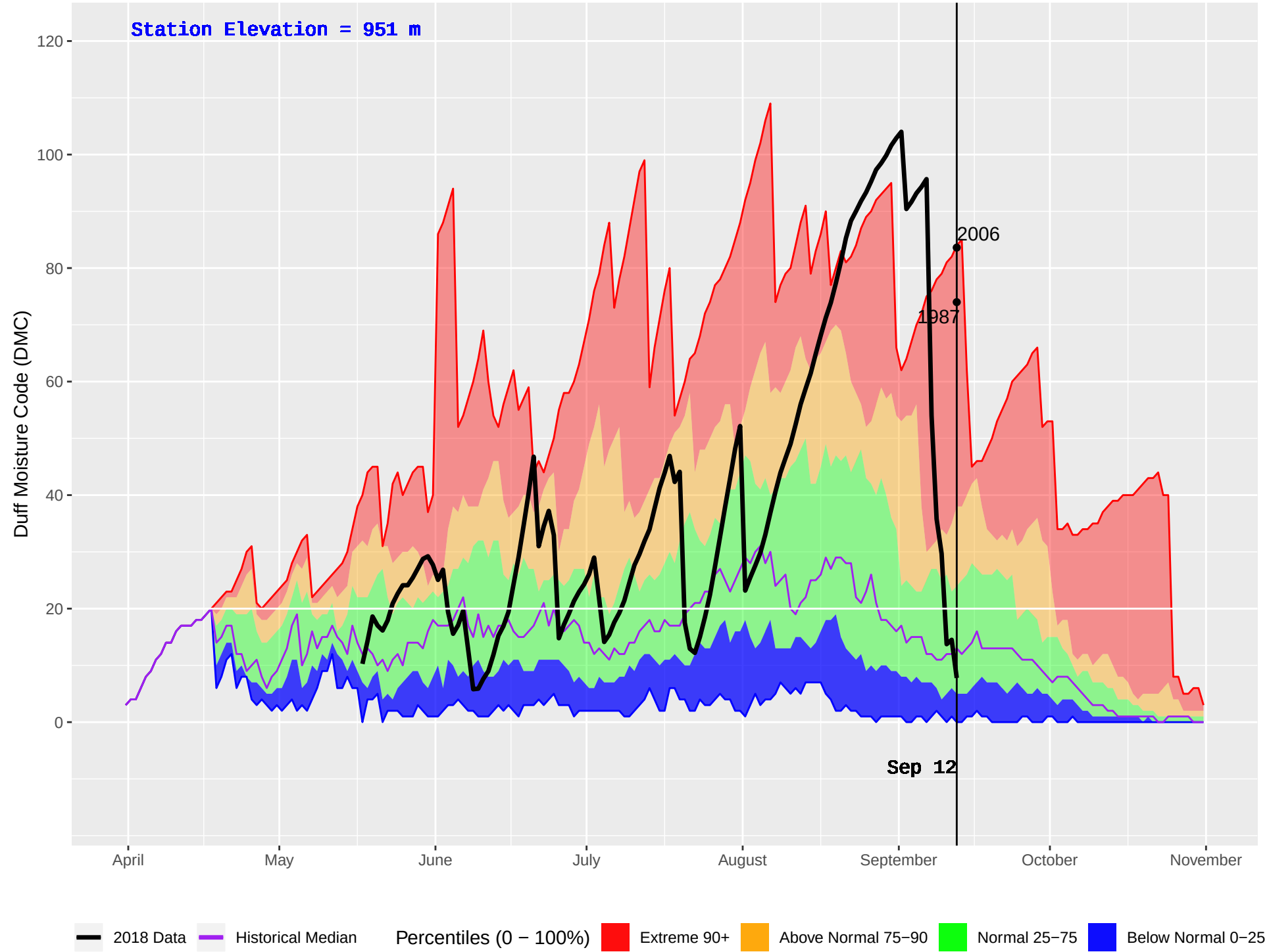
NORTH BABINE (173) : Historical (1986–2016) and Current (2018) Daily Duff Moisture Code (DMC)
