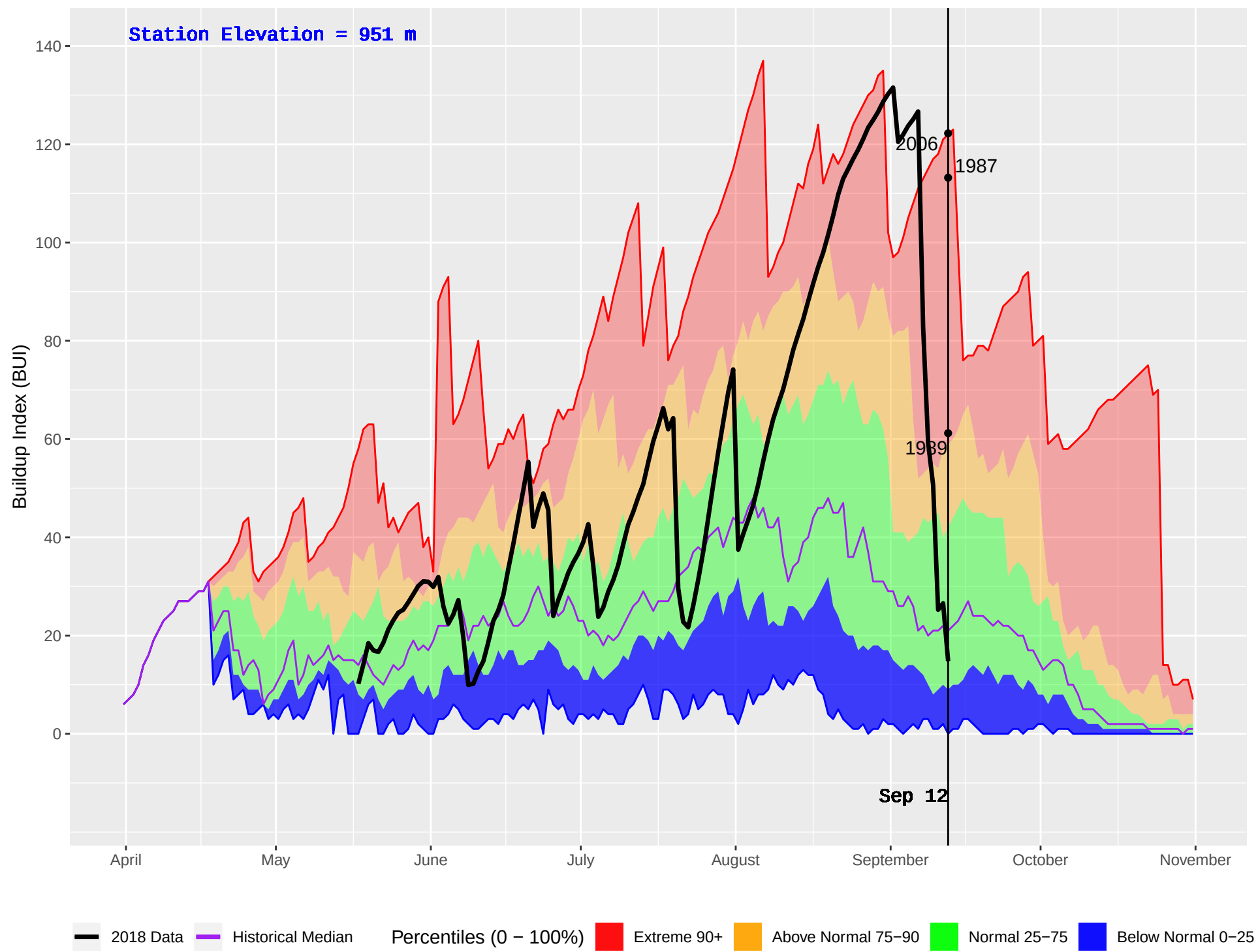
NORTH BABINE (173) : Historical (1986–2016) and Current (2018) Daily Buildup Index (BUI)
