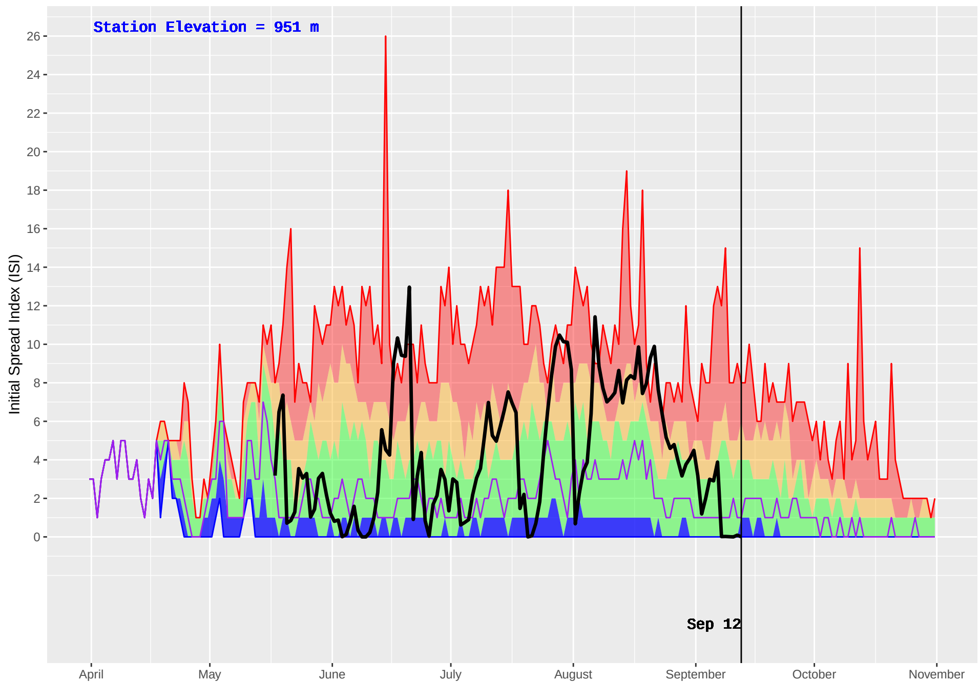
NORTH BABINE (173) : Historical (1986–2016) and Current (2018) Daily Initial Spread Index (ISI)
