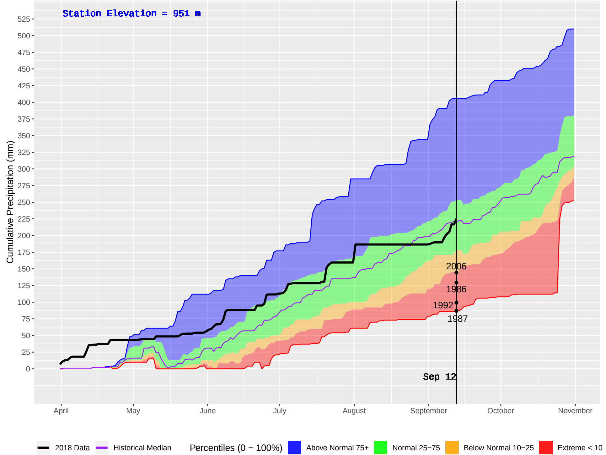
NORTH BABINE (173) : Historical (1986–2016) and Current (2018) Daily Cumulative Precipitation
